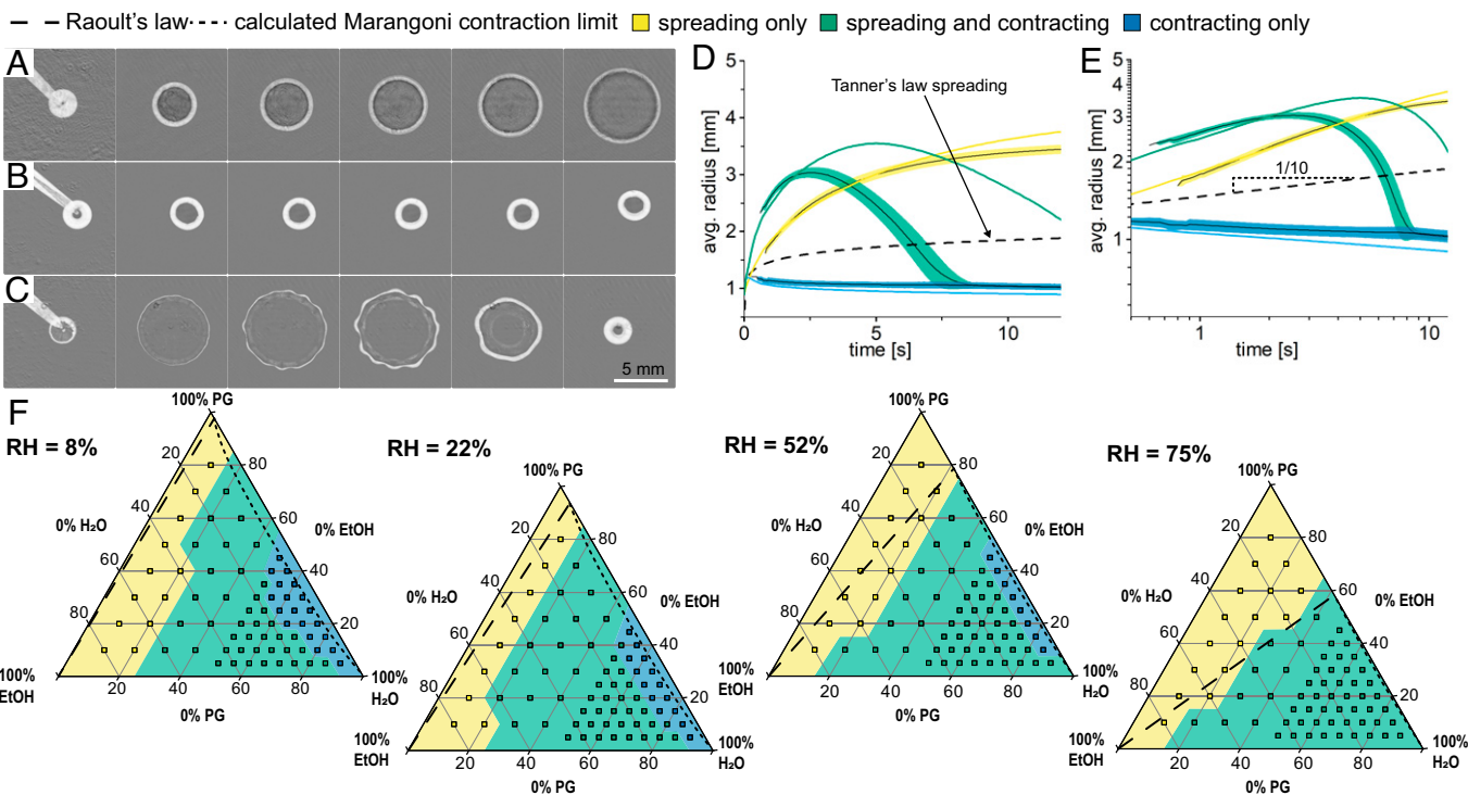
Fig. 1. Behaviors of ternary droplets on high-energy surfaces. (A–C) Time-series images ( t = 0, 1, 2, 3, 4 , and 10 s, at 52\% RH, in V/V_{tot} , V_{droplet} = 200 nL) of (A) enhanced spreading 10\% H 2 O/ 70\% PG/ 20\% EtOH, (B) contracting 70\% H 2 O/ 25\% PG/ 5\% EtOH, and (C) spreading and contracting 50\% H 2 O/ 30\% PG/ 20\% EtOH. (D and E) Radius vs. time plots of the mixtures in A–C with D linear and E log axes ( n = 10 ; SD shaded; solid colored lines correspond to the lubrication simulation). (F) The observable behaviors across the ternary parameter space at four different relative humidities. Overlaid are the theoretical considerations from Raoult's law (24) (dashed) and the net rate of change of the surface tension of the starting concentration (dotted). Avg., average.
