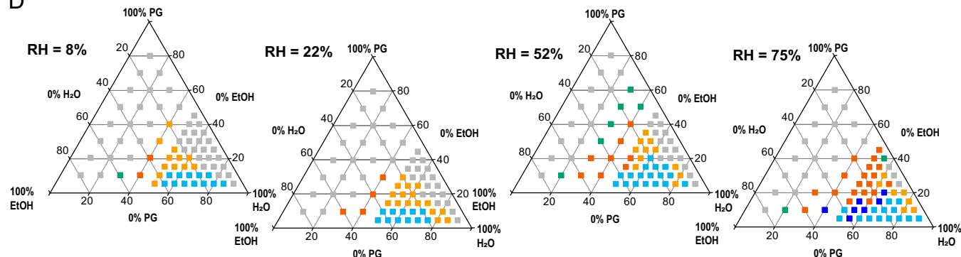
Fig. 3. Different forms of instabilities arising in ternary droplets. (A) Spreading instabilities of a droplet of 50% H 2 O/20% PG/30% EtOH at 52% RH. (B) Vigorous instabilities with chaotic satellite droplet formation of a droplet of 50% H 2 O/5% PG/45% EtOH at 44% RH. (C) Rivulet formation during the contracting phase of a droplet of 30% H 2 O/10% PG/60% EtOH at 22% RH. (D) Observed instability formation across the ternary phase space at different humidities. Time lapses of A–C are shown in SI Appendix, Fig. S5 and Movie S4 . V_{\text{droplet}} = 200 nL for A and C and 100 nL for B, respectively.
